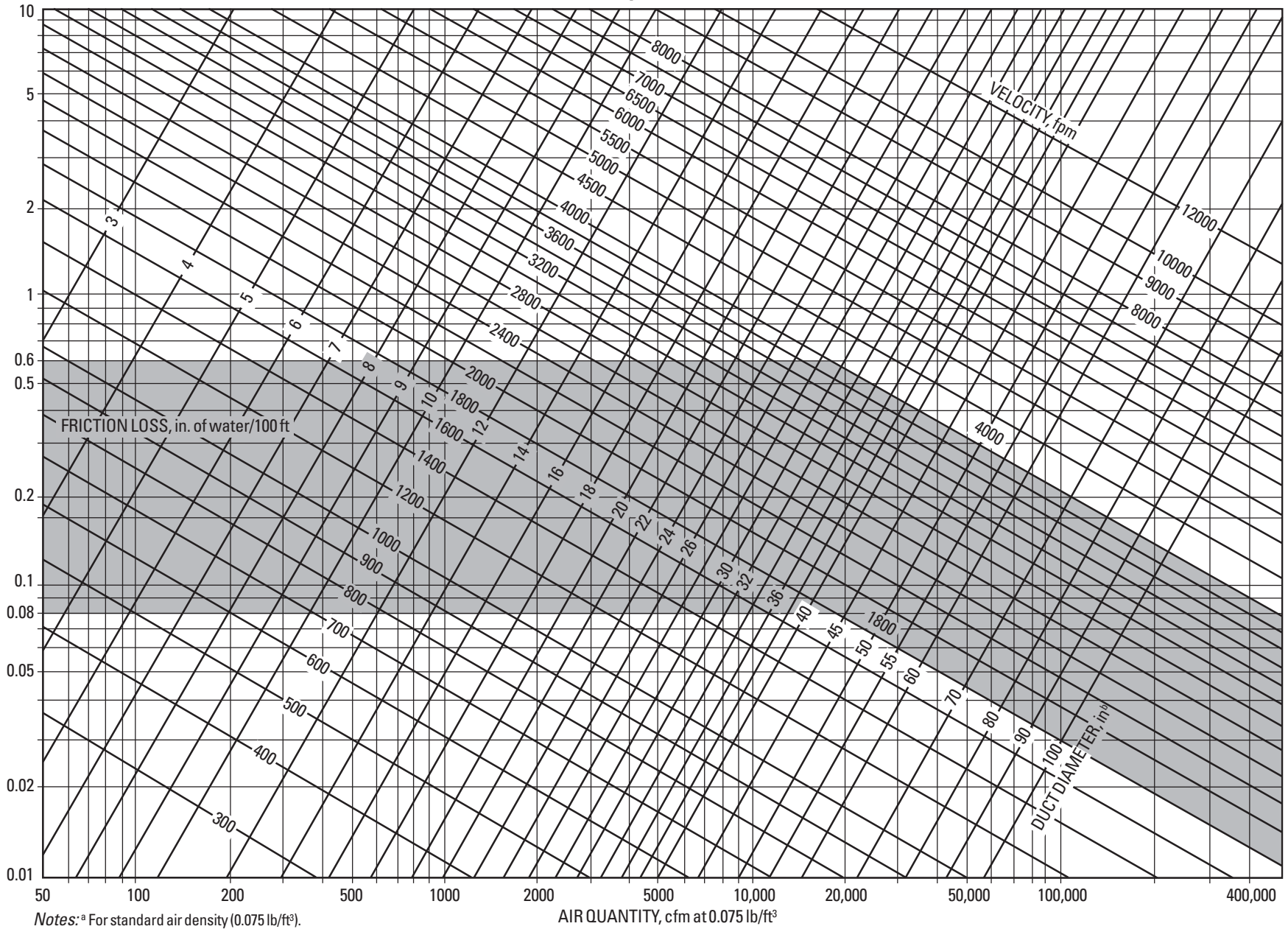
Example airflow chart a
